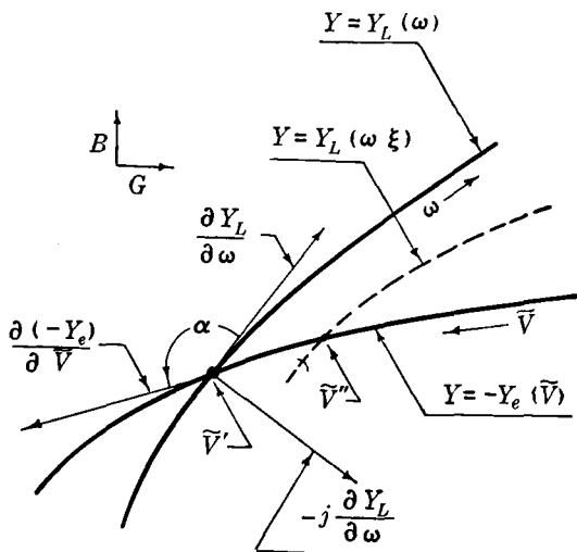
FIG. 7-8.—Stability diagram on the basis of the load and operating curves. The condition for stability is that the angle \alpha , between the vectors \partial Y_L/\partial \omega and \partial(-Y_e)/\partial \bar{V} , measured in a counterclockwise direction, must lie between 0^\circ and 180^\circ .
